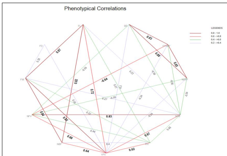
Fig. 1. Pictorial representation of phenotypic correlation coefficients of F 2 population "HUB-1 × CO-1" in bitter Gourd.
