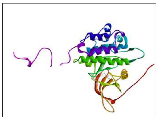
(A) The EGFR protein with the ligand Topotecan and its interacting residues
