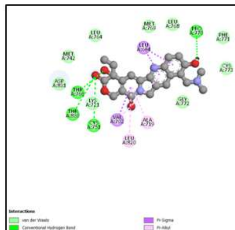
(A) The EGFR protein with the ligand Topotecan and its interacting residues
