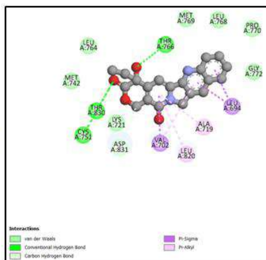
(C) The EGFR protein with the ligand Camptothecin and its interacting residues
