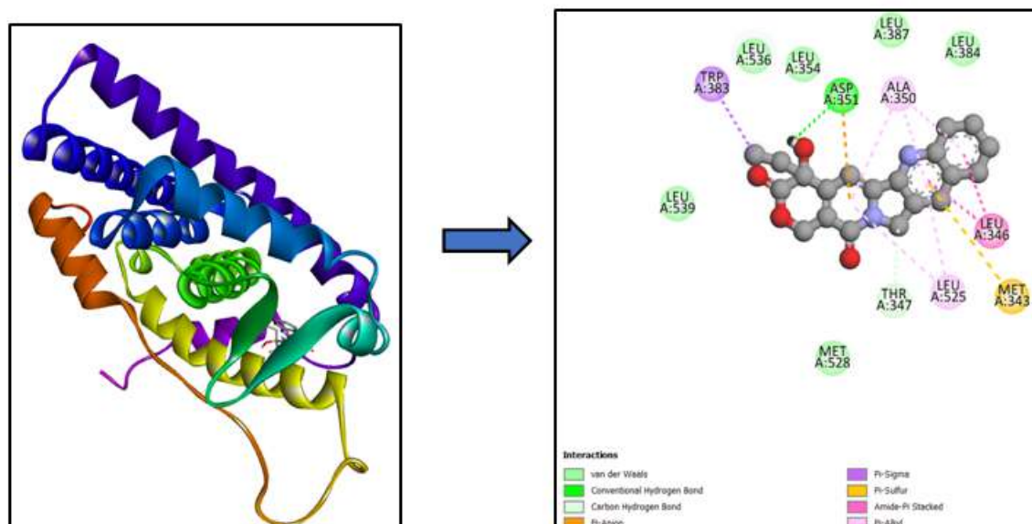
(C) The ER- \alpha protein with the ligand Camptothecin and its interacting residues Fig. 4. The ER- \alpha protein with its interacting residues.
