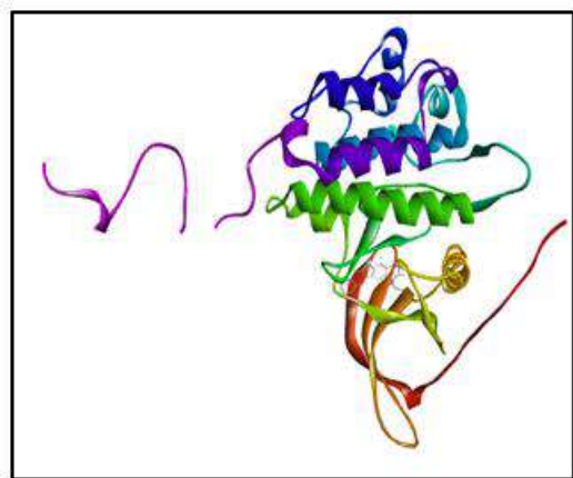
(C) The EGFR protein with the ligand Camptothecin and its interacting residues
