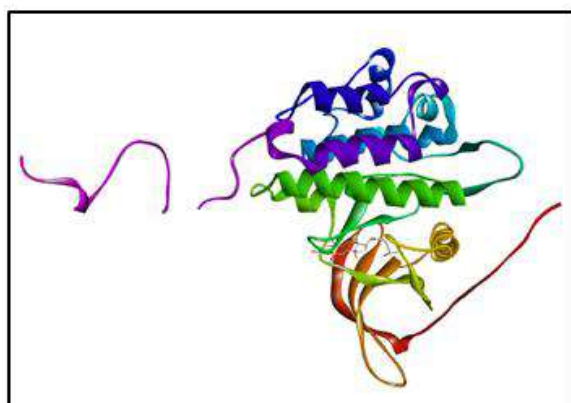
(B) The EGFR protein with the ligand Macdougallin and its interacting residues
