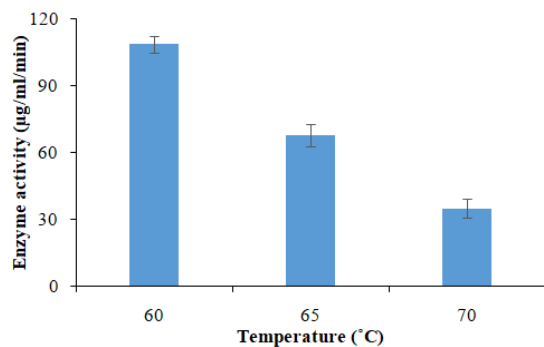
Fig. 3. Thermo-stability of the produced \alpha -amylase enzyme at different temperatures.
