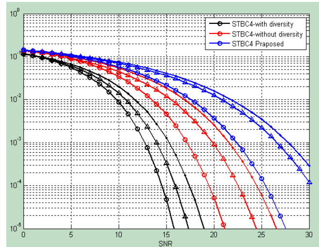
Fig. 3. BER vs SNR for Performance of the system with, without, and proposed diversity for various antennas.
