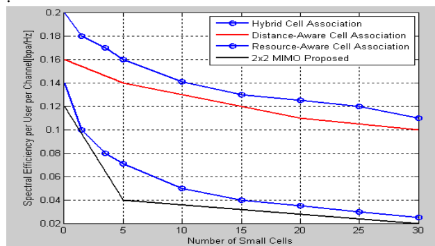
Fig. 4. Performance 2x2 MIMO Proposed.
