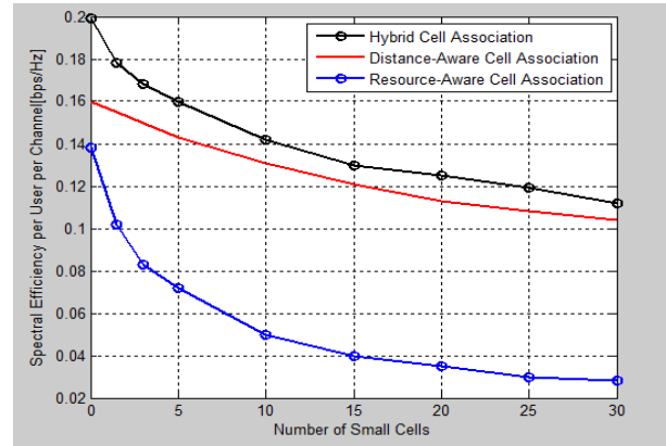
Fig. 6. Hybrid cell association scheme Combine resource-aware and distance-aware criteria A user selects a cell with the maximum of product of distance-based channel gain and p_i . If p_i = 0 (i.e., high or innate traffic load), a user will not select cell i even if it is the closest cell and vice versa. Hybrid scheme achieves a balance between traffic load balancing and throughput maximization. Quantitative comparison among resource-aware, distance-aware, and hybrid cell association schemes: two-tier macrocell-small cell network, downlink transmission, round-robin scheduling.
