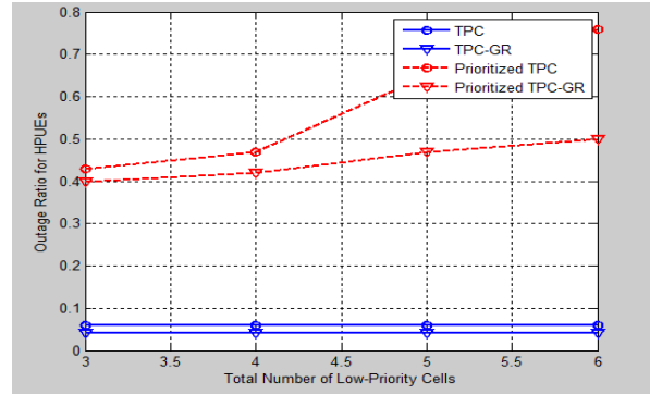
Fig. 5. Performance Prioritized power control A two-tier system (high-priority cell tier and low-priority cell tier) with same target SIR for all users 5 HPUEs per high-priority cell and 4 LPUEs per low-priority cell, each user is associated with only one BS of its corresponding tier. LPUEs employ either TPC, TPC-GR, prioritized TPC, or prioritized TPC-GR, and HPUEs use TPC (i.e., rigidly track their target-SIRs). Although outage ratio for HPUEs are improved by TPC-GR, as compared to TPC, protection of HPUEs is not guaranteed. Prioritized TPC and TPC-GR guarantee protection of HPUEs at the cost of increased outage ratio for LPUEs. Also, with prioritized OPC for LPUEs and TPC for HPUEs, protection of HPUEs is guaranteed at the cost of decreased throughput for LPUEs (compared to non-prioritized OPC).
