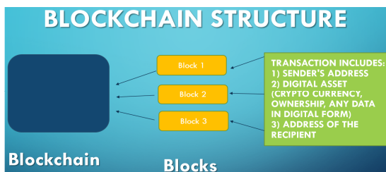
Fig. 1. Blockchain structure.
