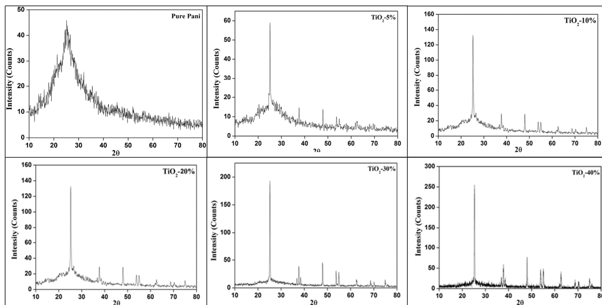
Fig. 1. X-ray diffraction patterns of Pure Polyaniline and TiO 2 / PANI (5%, 10%, 20%, 30%, 40%).
