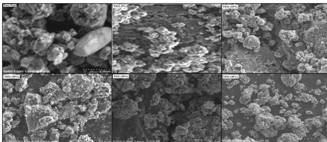
Fig. 2. SEM micrographs of Pure Polyaniline and TiO 2 doped with 5%, 10%, 20%, 30%, 40%.
