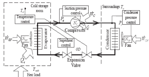
Fig. 2. Schematic layout of basic refrigeration system.
