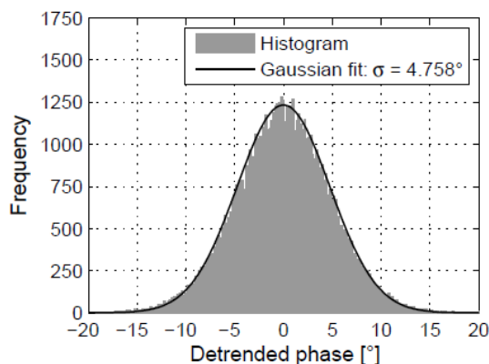
Fig. 1. Distribution of the detrended phase for 3 range and 12 azimuth looks (0.5 x 0.621 m sample interval), using the ML method. All verification areas were combined to produce the figure. The histogram used a 0.2° bin width.
