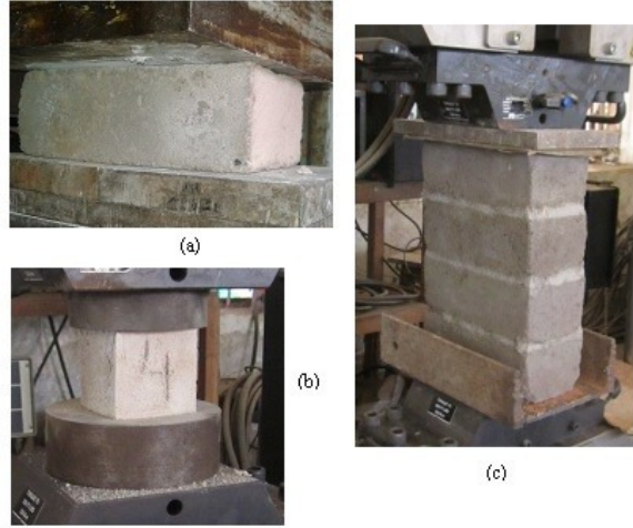
Fig. 3. Test setup for Crushing strength.
