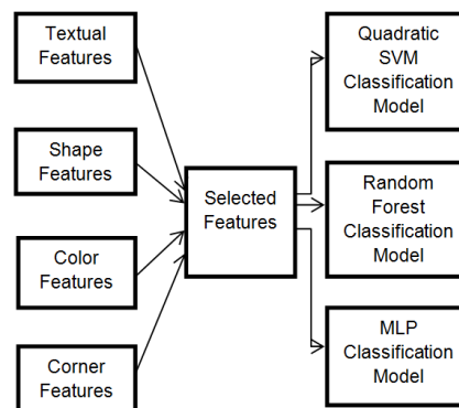
Fig. 2. Feature Selection and reduction hierarchy.
