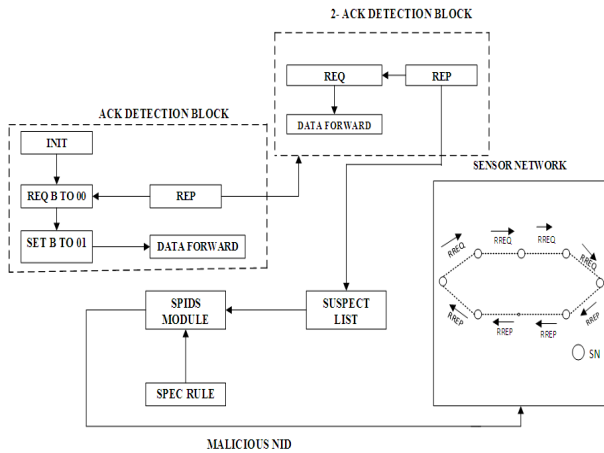
Fig. 1. IDS architecture.
