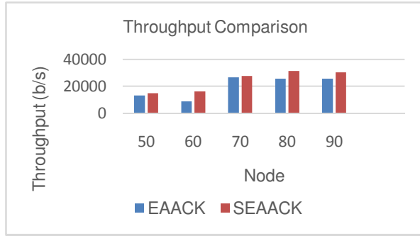
Fig. 7. Throughput comparison.
